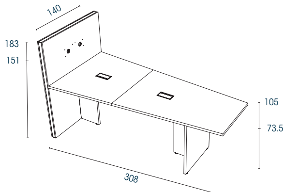
Panel legs
