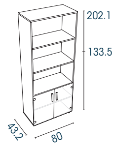
2 glass doors
