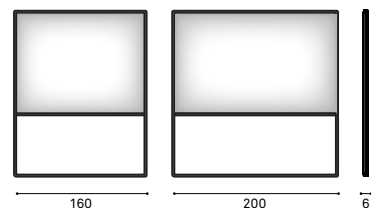
Whiteboard + upholstered panel/decor panel
