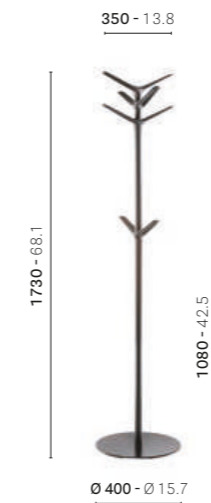
5144B Coat stand, steel bar and polypropylene arms
