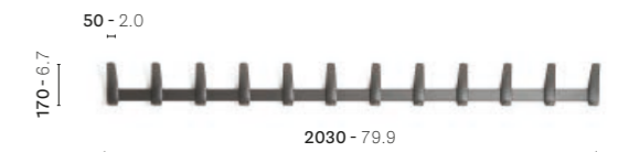
5150W12 Coat hanger, steel bar and polypropylene hooks
