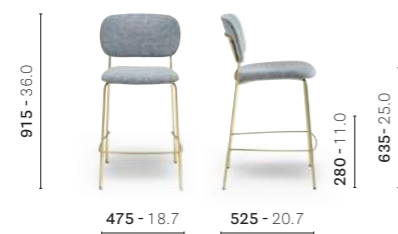
3708 Barstool, upholstered seat and back, steel tube frame
