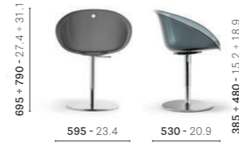
951 Armchair, polycarbonate shell, steel central base
