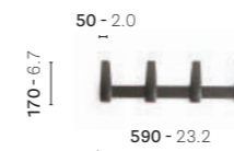
5150W4 Coat hanger, steel bar and polypropylene hooks
